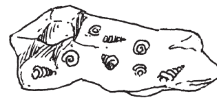
Sedimentary / Limestone
