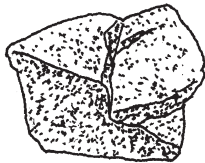
Metamorphic / Gneiss
