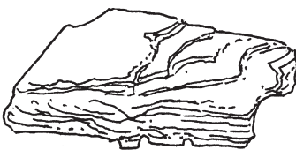
Sedimentary / Sandstone
