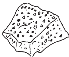
Igneous / Granite
